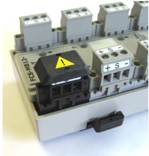
FCS-A10 installed on Megablock Trunk
